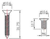
12# Wooden screw
